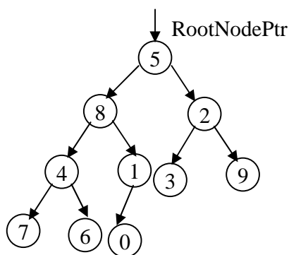
Construct the initial binary tree
